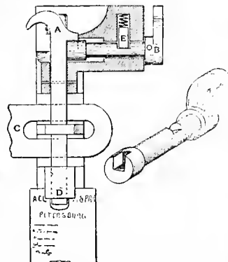
Fig. 3898a. SULLY'S SEAL-LOCK.
